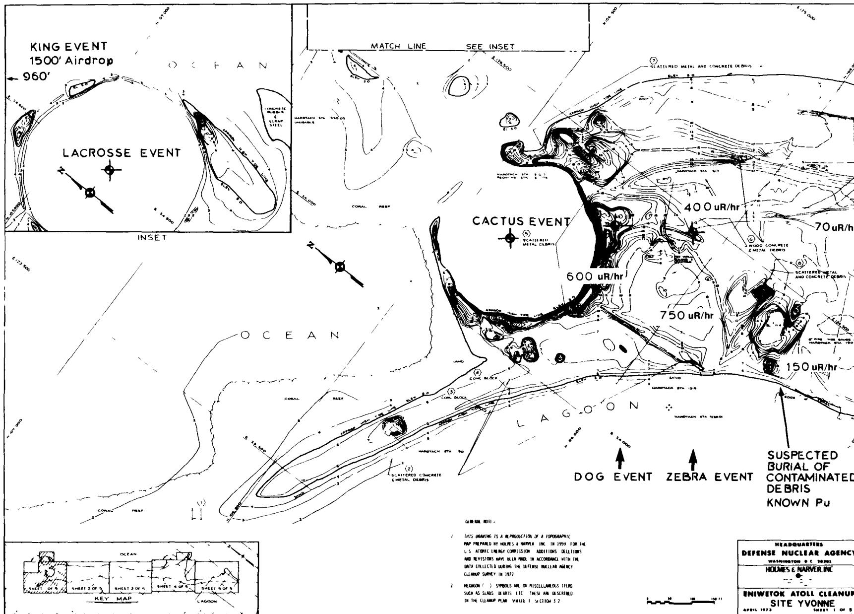
FIGURE 68 SITE YVONNE, SHEET 1 OF 5
